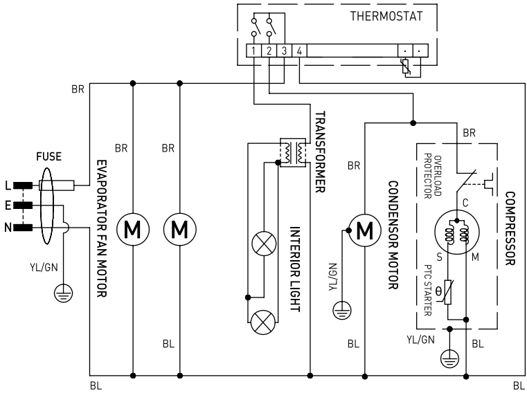
Circuit diagram (233931)
