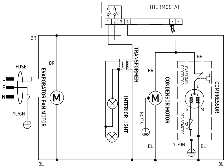
Circuit diagram (233924)
